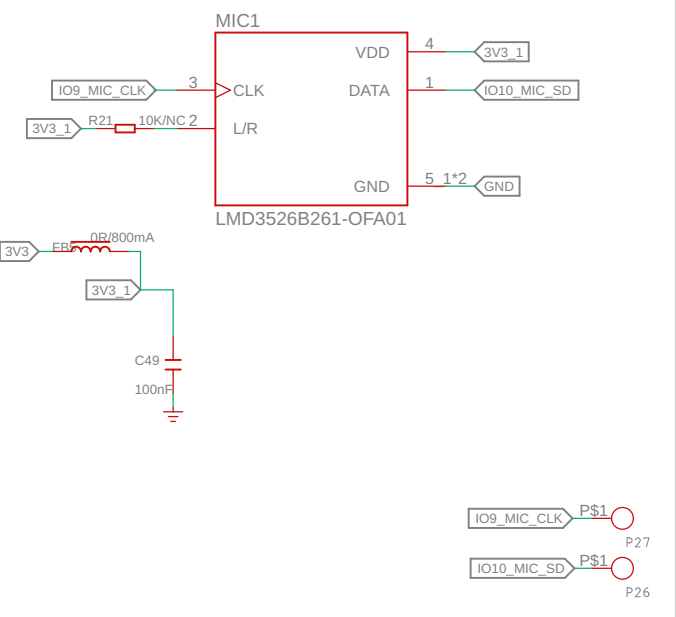
I2S MIC
