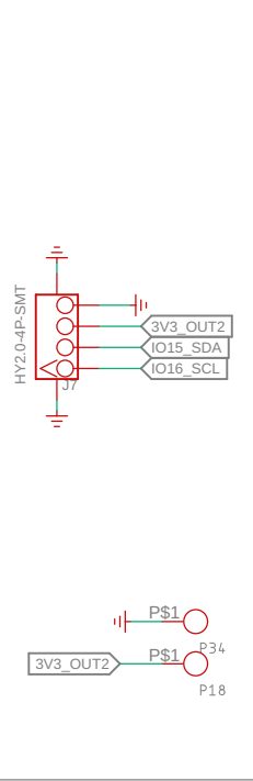
3.3V-I2C Output
